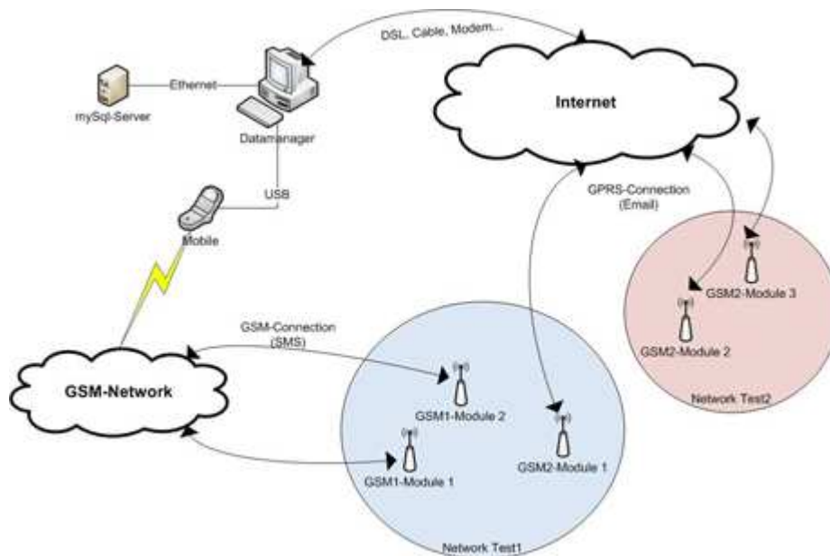
Illustration of the GSM-2 measuring system
