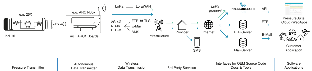
Remote transmission with LoRaWAN or NB-IoT networks
